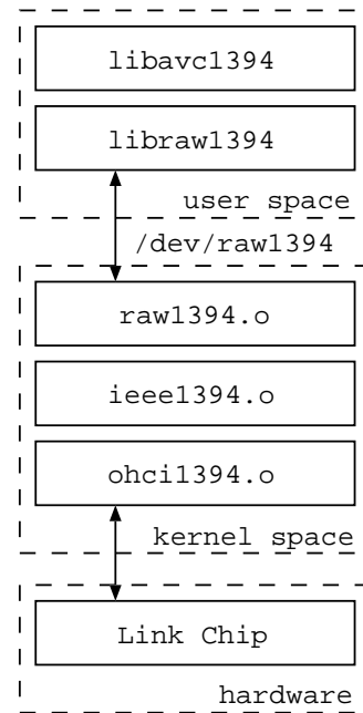
Figure 4. IEEE1394 API for Linux
