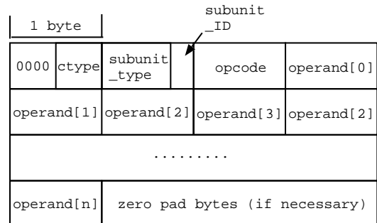
Figure 3. AV/C Protocol Frame
